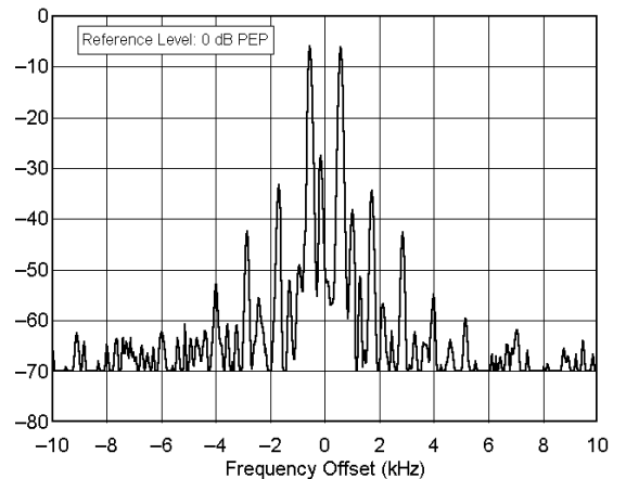
Yaesu FT-847 sn 8C020205 18.120 MHz, Transmit IMD, 100 W F:\SHARED\PROD_REV\TESTS\FT847\FT847117.TXT
