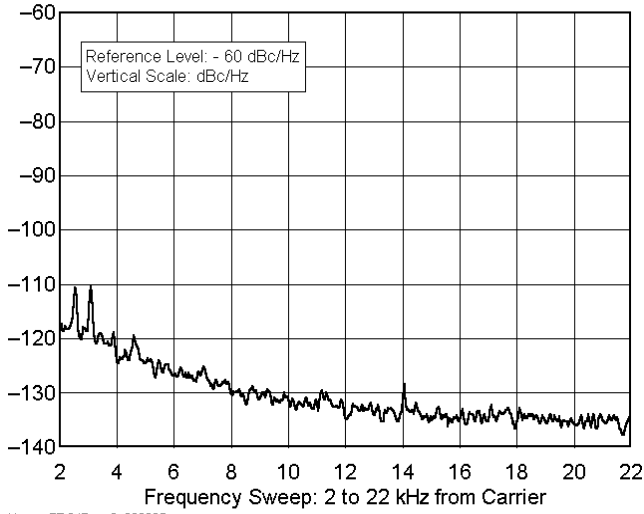
Yaesu FT-847 sn 8c020205 3.520 MHz, Phase Noise, 100 W F:\SHARED\PROD_REVTESTS\FT847\FT847P80.TXT
