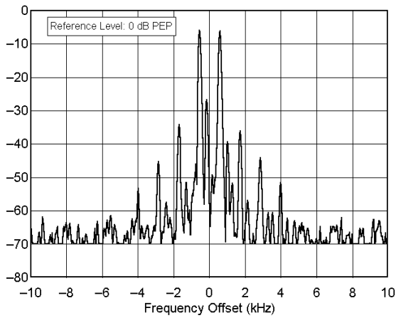
Yaesu FT-847 sn 8C020205 21.250 MHz, Transmit IMD, 100 W F:\SHARED\PROD_REV\TESTS\FT847\FT847115.TXT
