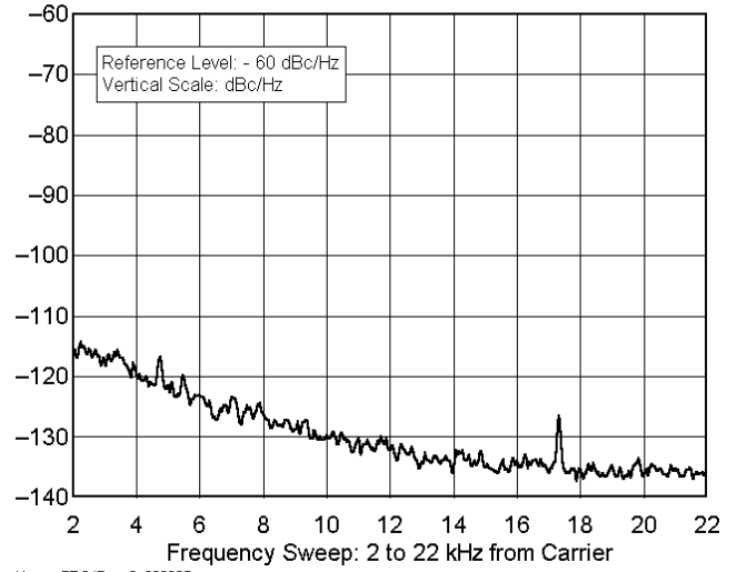
Yaesu FT-847 sn 8c020205 50.020 MHz, Phase Noise, 100 W F:\SHARED\PROD_REVTESTS\FT847\FT847P6M.TXT
