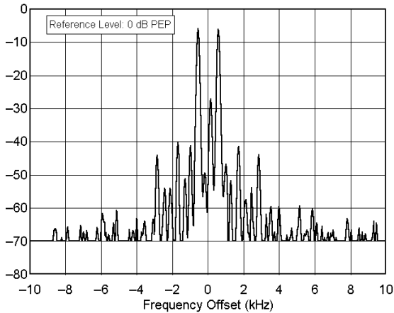
Yaesu FT-847 sn 8C020205 3.900 MHz, Transmit IMD, 100 W F:\SHARED\PROD_REV\TESTS\FT847\FT847160.TXT
