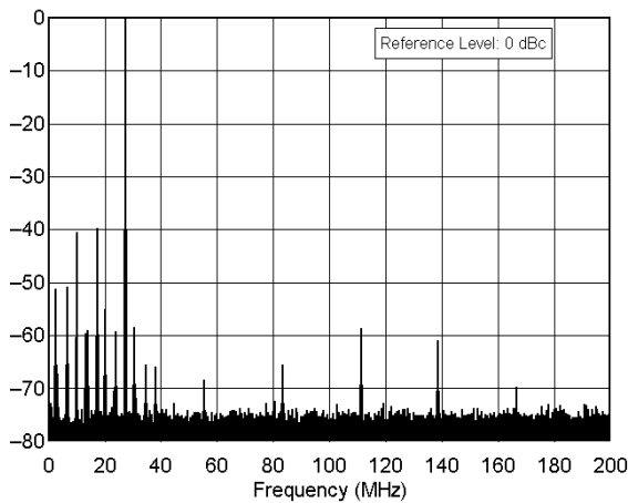
Yaesu FT-847 sn 8C020205 28.0 MHz Band, Spectral Purity, 100 W F:\SHARED\PROD_REV\TESTS\F1847\F1847S10.TXT
