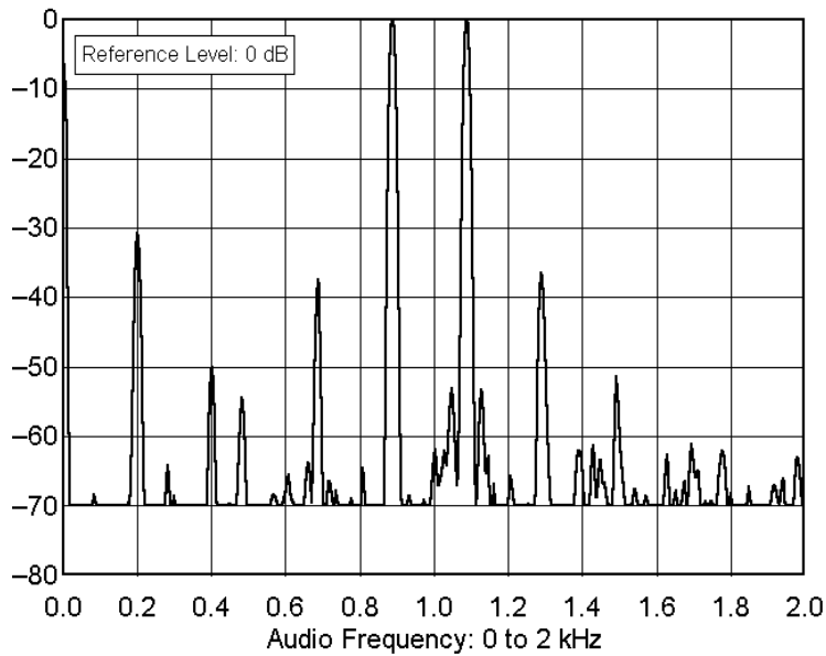
Yaesu FT-847 serial number 8C020205 14.020 MHz, AGC Fast, In-Band Receiver IMD F:\SHARED\PROD_REV\TESTS\FT847\FT847IBF.TXT
