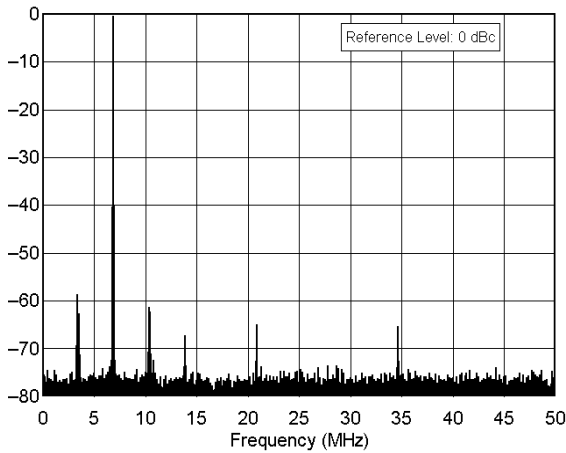
Yaesu FT-847 sn 8C020205 7.0 MHz Band, Spectral Purity, 100 W F:\SHARED\PROD_REV\TESTS\F847\F847S40.TXT
