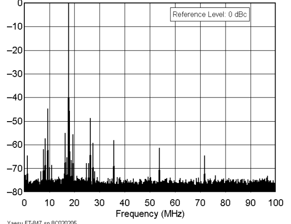
Yaesu FT-847 sn 8C020205 18.1 MHz Band, Spectral Purity, 100 W F:\SHARED\PROD_REV\TESTS\F847\F847S17.TXT
