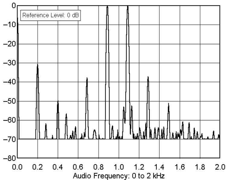
Yaesu FT-847 serial number 8C020205 14.020 MHz, AGC Slow, In-Band Receiver IMD F:\SHARED\PROD_REV\TESTS\FT847\FT847IBS.TXT
