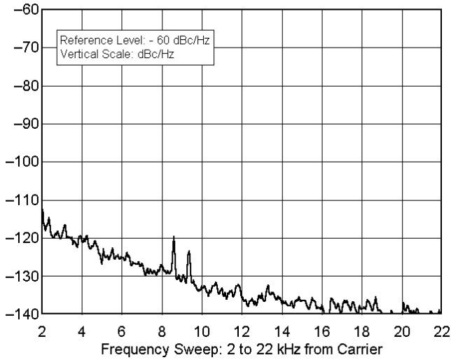
Yaesu FT-847 sn 8c020205 14.020 MHz, Phase Noise, 100 W F:\SHARED\PROD_REVTESTS\FT847\FT847P20.TXT
