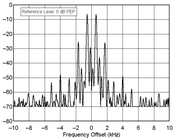
Yaesu FT-847 sn 8C020205 28.350 MHz, Transmit IMD, 100 W F:\SHARED\PROD_REV\TESTS\FT847\FT847110.TXT
