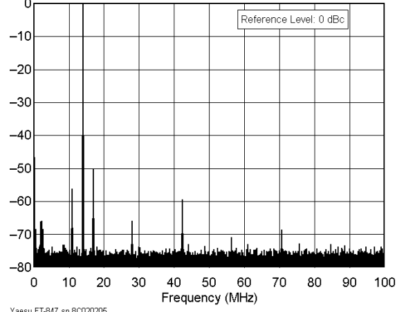
Yaesu FT-847 sn 8C020205 14.0 MHz Band, Spectral Purity, 100 W F:\SHARED\PROD_REV\TESTS\F847\F847S20.TXT
