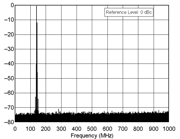
Yaesu FT-847 sn 8C020205 144.0 MHz Band, Spectral Purity, 100 W F:\SHARED\PROD_REV\TESTS\F1847\F1847S2M.TXT
