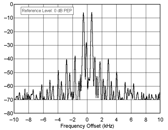
Yaesu FT-847 sn 8C020205 50.200 MHz, Transmit IMD, 100 W F:\SHARED\PROD_REV\TESTS\FT847\FT84716M.TXT
