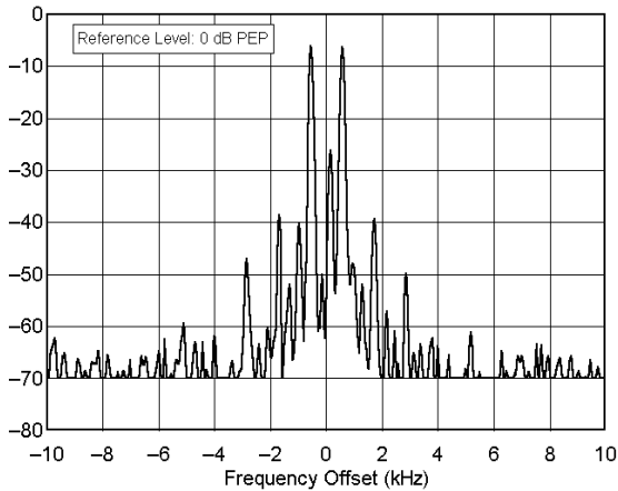
Yaesu FT-847 sn 8C020205 7.250 MHz, Transmit IMD, 100 W F:\SHARED\PROD_REV\TESTS\FT847\FT847140.TXT
