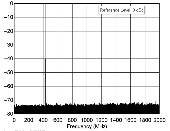
Yaesu FT-847 sn 8C020205 420.0 MHz Band, Spectral Purity, 50 W F:\SHARED\PROD_REV\TESTS\F1847\F1847S70.TXT
