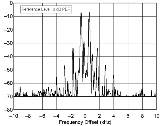
Yaesu FT-847 sn 8C020205 14.250 MHz, Transmit IMD, 100 W F:\SHARED\PROD_REV\TESTS\FT847\FT847120.TXT
