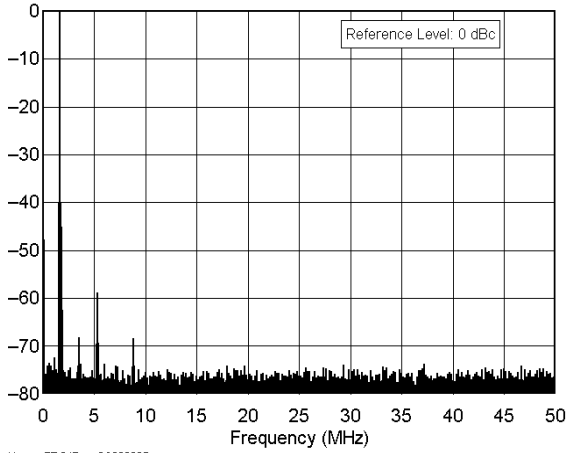
Yaesu FT-847 sn 8C020205 1.8 MHz Band, Spectral Purity, 100 W F:\SHARED\PROD_REV\TESTS\F847\F847S10.TXT
