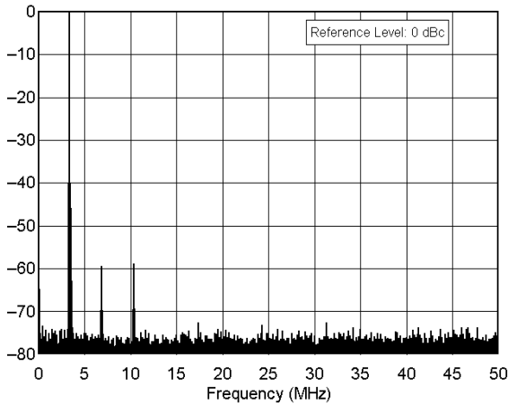
Yaesu FT-847 sn 8C020205 3.5 MHz Band, Spectral Purity, 100 W F:\SHARED\PROD_REV\TESTS\F847\F847S80.TXT
