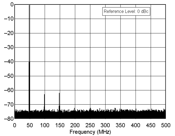
Yaesu FT-847 sn 8C020205 50.0 MHz Band, Spectral Purity, 100 W F:\SHARED\PROD_REV\TESTS\F1847\F1847S6M.TXT
