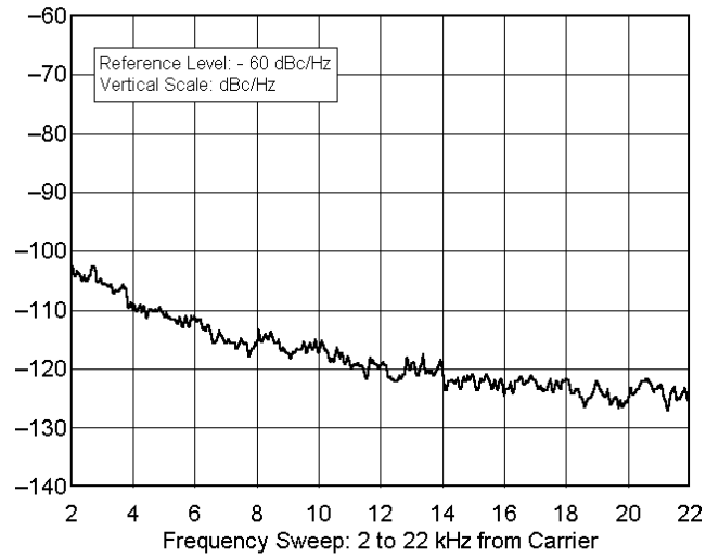
Yaesu FT-847 sn 8c020205 144.020 MHz, Phase Noise, 100 W F:\SHARED\PROD_REVTESTS\FT847\FT847P2M.TXT
