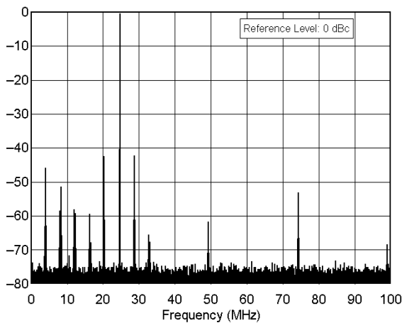
Yaesu FT-847 sn 8C020205 24.9 MHz Band, Spectral Purity, 100 W F:\SHARED\PROD_REV\TESTS\F1847\F1847S12.TXT
