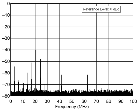
Yaesu FT-847 sn 8C020205 21.0 MHz Band, Spectral Purity, 100 W F:\SHARED\PROD_REV\TESTS\F1847\F1847S15.TXT
