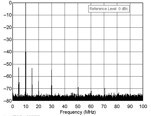
Yaesu FT-847 sn 8C020205 10.1 MHz Band, Spectral Purity, 100 W F:\SHARED\PROD_REV\TESTS\F847\F847S30.TXT
